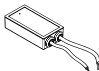
Power supply 16W 110-240V IP65 125x61x31mm
