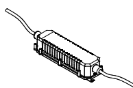
Power supply 24V DC 70W IP67 267x79x52mm
