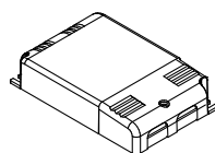
Power supply 24V 20Watt IP20 103x67x21mm
