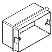
Recessed box Modulo A RC 74x106x53,5mm
